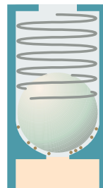
Fig. 13: By-pass valve
